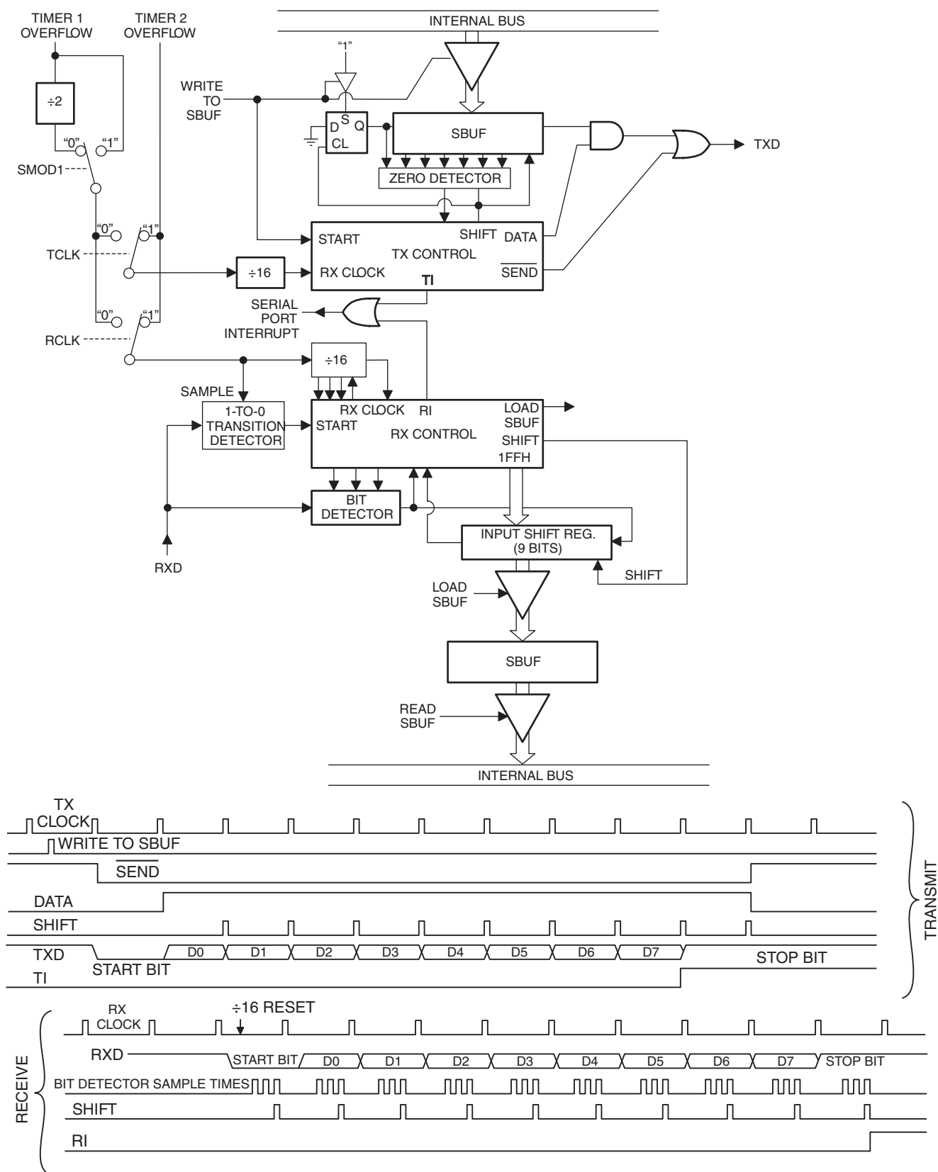
Figure 14-6. Serial Port Mode 1
