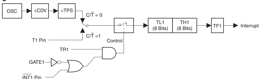
Figure 11-2. Timer/Counter 1 Mode 1: 16-bit Counter
