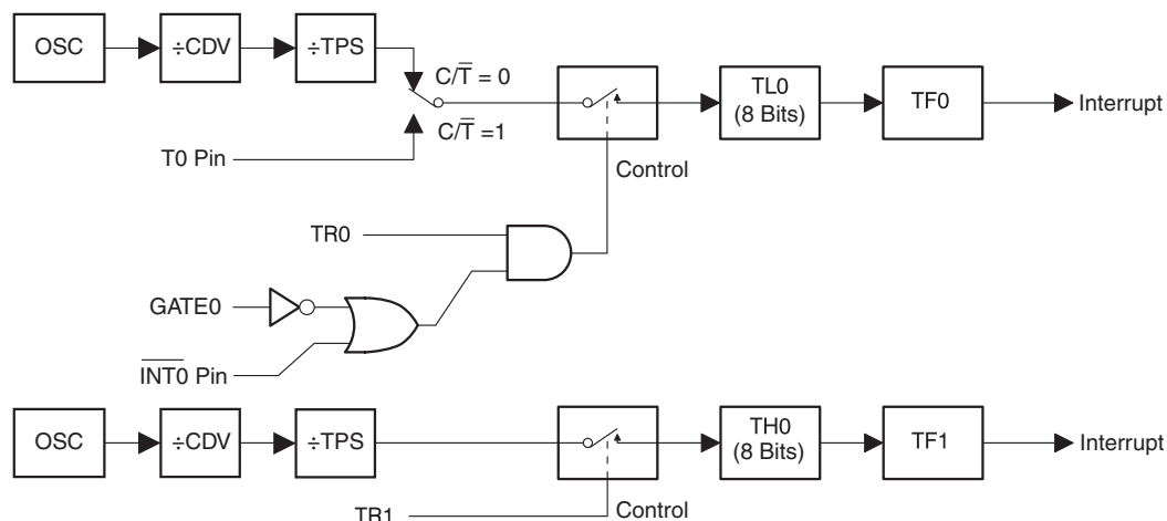
Figure 11-4. Timer/Counter 0 Mode 3: Two 8-bit Counters
