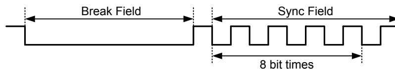
Figure 24-12. LIN Break and Sync Fields
