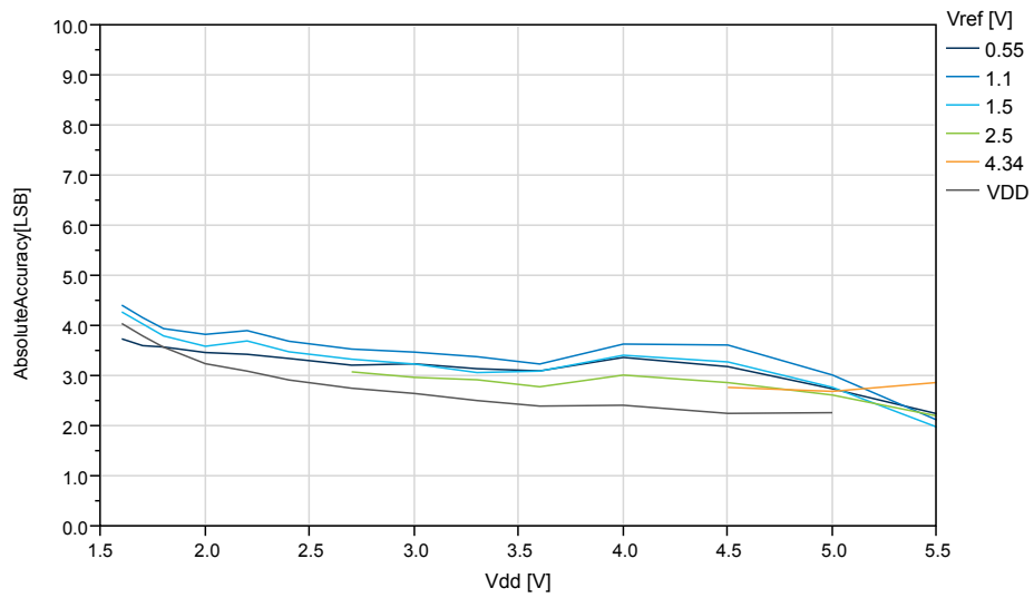
Figure 35-42. Absolute Accuracy vs. V_{DD} (115ksps) at T=25^{\circ}\text{C}
