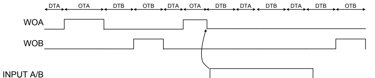
Figure 22-16. Input Mode 5
