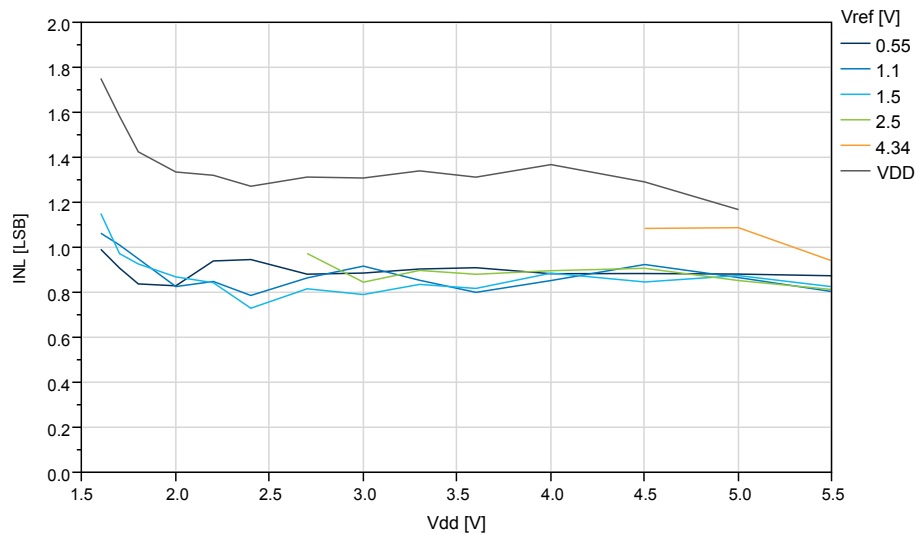
Figure 35-48. INL vs. V_{DD} (115ksps) at T=25^{\circ}\text{C}
