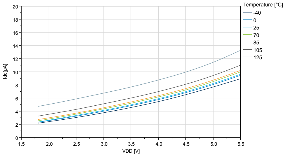
Figure 35-9. Idle Supply Current vs. V_{DD} (f=32KHz OSCULP32K)
