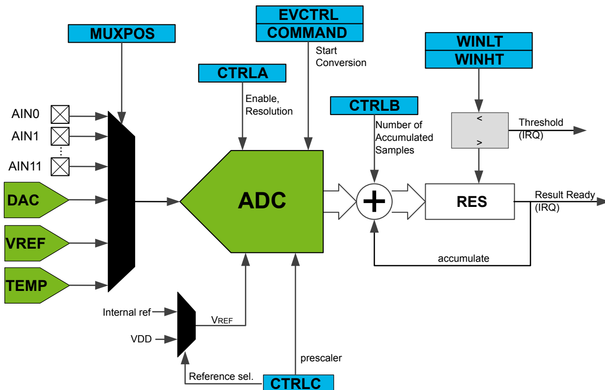
Figure 30-1. Block Diagram
