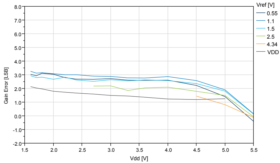
Figure 35-47. Gain Error vs. V_{ref} ( V_{DD}=5.0\text{V} , 115ksps)
