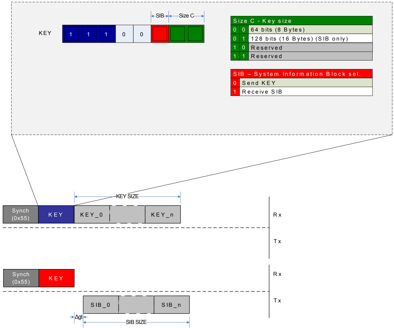
Figure 33-16. KEY Instruction Operation
