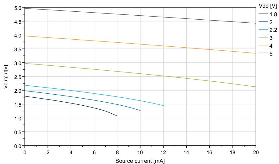
Figure 35-28. IO Pin Output Voltage vs. Source Current ( T=25^{\circ}C )
