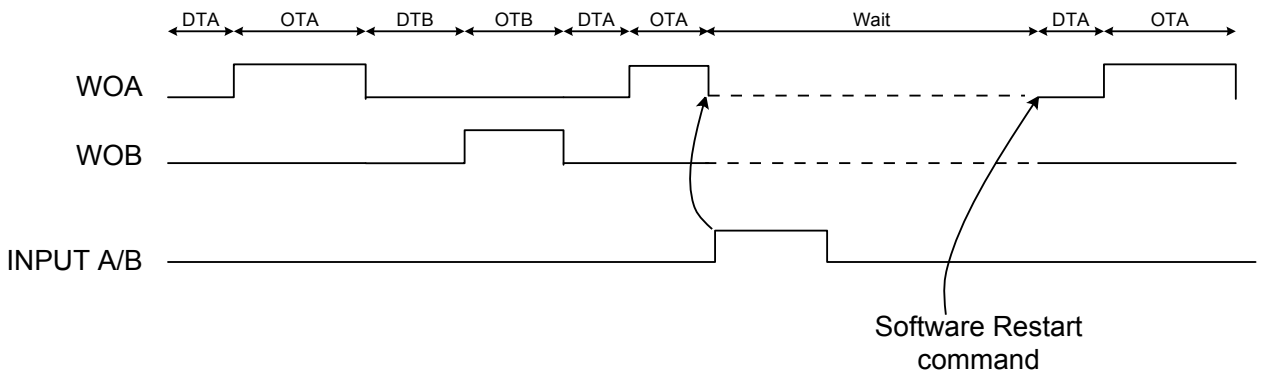
Figure 22-18. Input Mode 7
