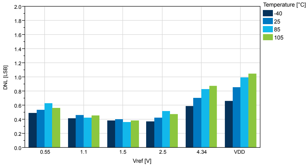
Figure 35-45. DNL vs. V_{ref} ( V_{DD}=5.0V , 115kps)
