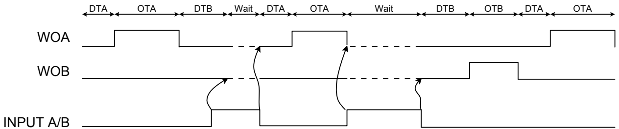
Figure 22-17. Input Mode 6
