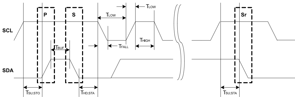
Figure 26-14. SCL Timing
