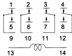
WIRING DIAGRAM
