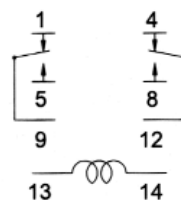
WIRING DIAGRAM
