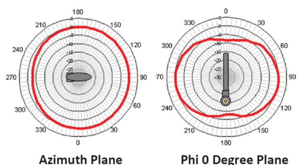
960 MHz
