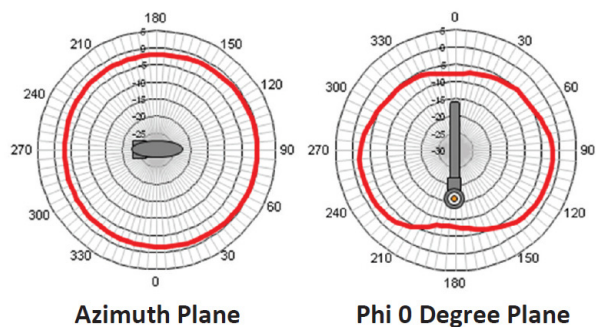
824 MHz
