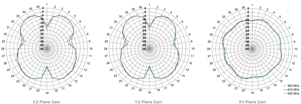
Figure 16. Radiation Patterns for ANT-8/9-IPW3-NP Antenna, Center of Ground Plane
