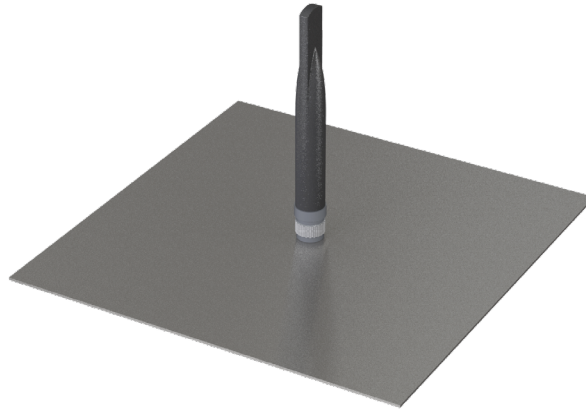
Figure 10. ANT-8/9-IPW3-NP at Center of Ground Plane
