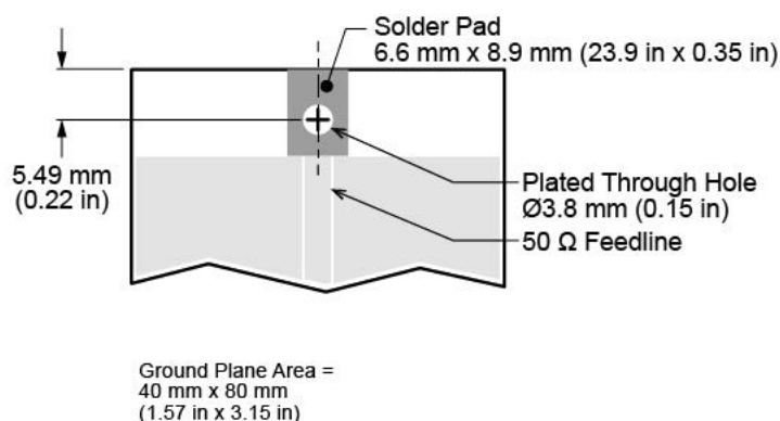
Figure 2. ANT-8/9-PW-LPN Recommended Mounting and PCB Footprint
