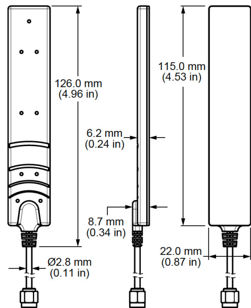
Figure 1. ANT-2/5-VDP-2000 Antenna
