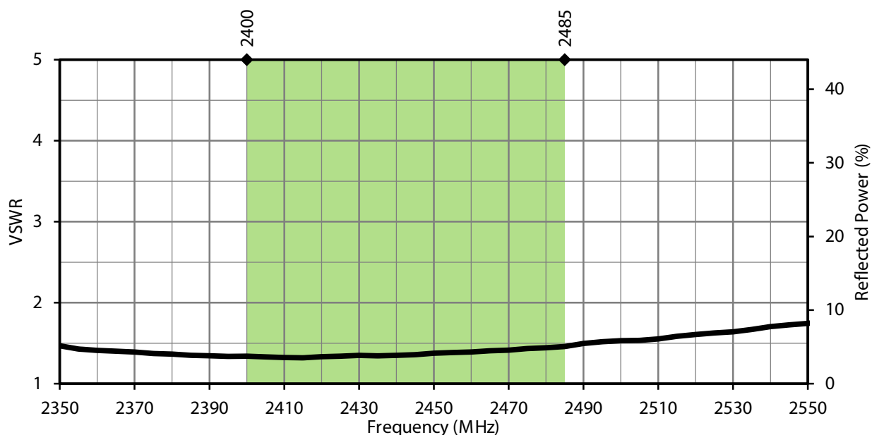
Figure 3. LPW VSWR, Bent-90
