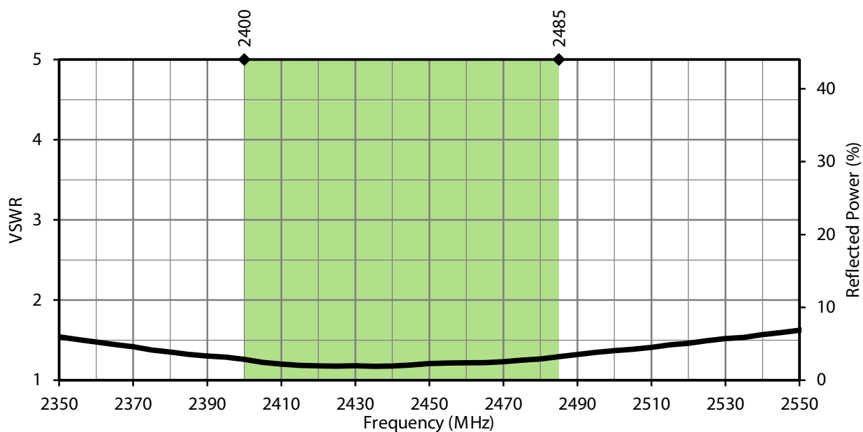
Figure 10. LPW VSWR, Straight
