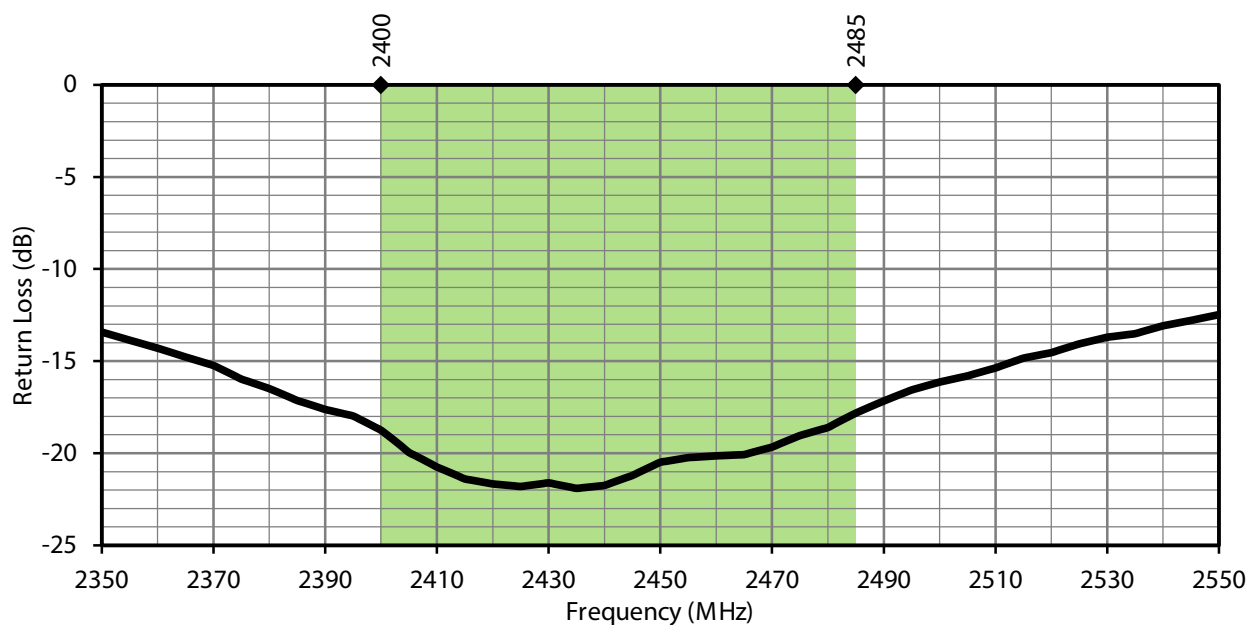
Figure 11. LPW Return Loss, Straight
