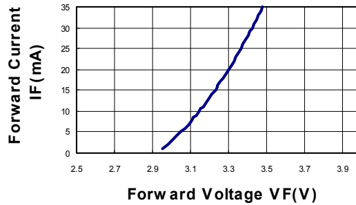
Forward Current vs Forward Voltage
