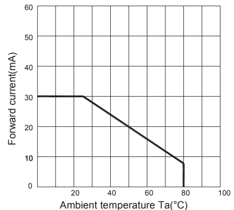
Fig.5 Forward current derating curve vs. Ambient temperature
