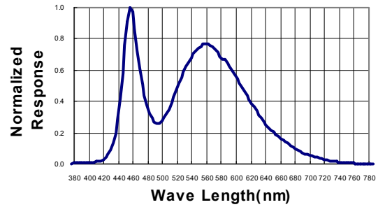
Spectral Radiance
