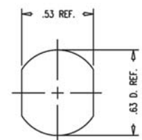
MOUNTING HOLE AO
