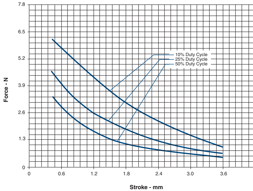
Typical Force @ 20°C (Net, with Spring)
