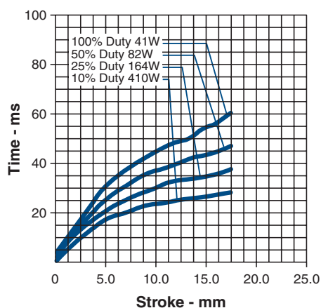
Size 8ECM— Typical Speed @ No Load, 20°C
