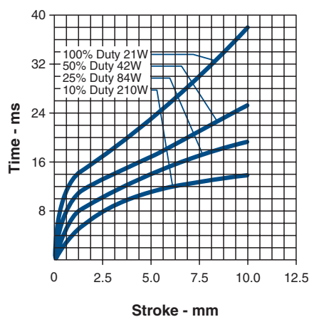
Size 5ECM— Typical Speed @ No Load, 20°C
