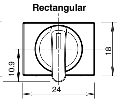
[Lever Operator]
