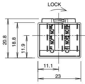
[3PDT]
