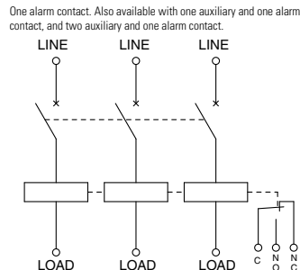
NC1V-3121 (With alarm contact)
