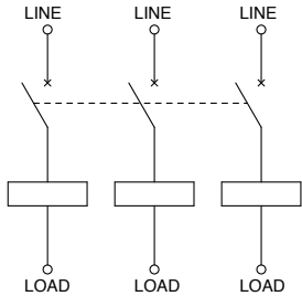
NC1V-3100 (Without auxiliary/alarm contacts)
