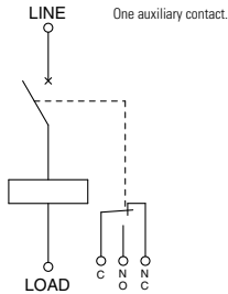
NC1V-1111 (With auxiliary contact)
