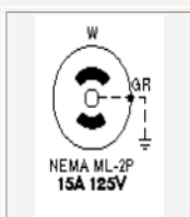
NEMA Configuration
