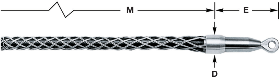
Fiber Optic Pulling Grip, Swivel Eye
