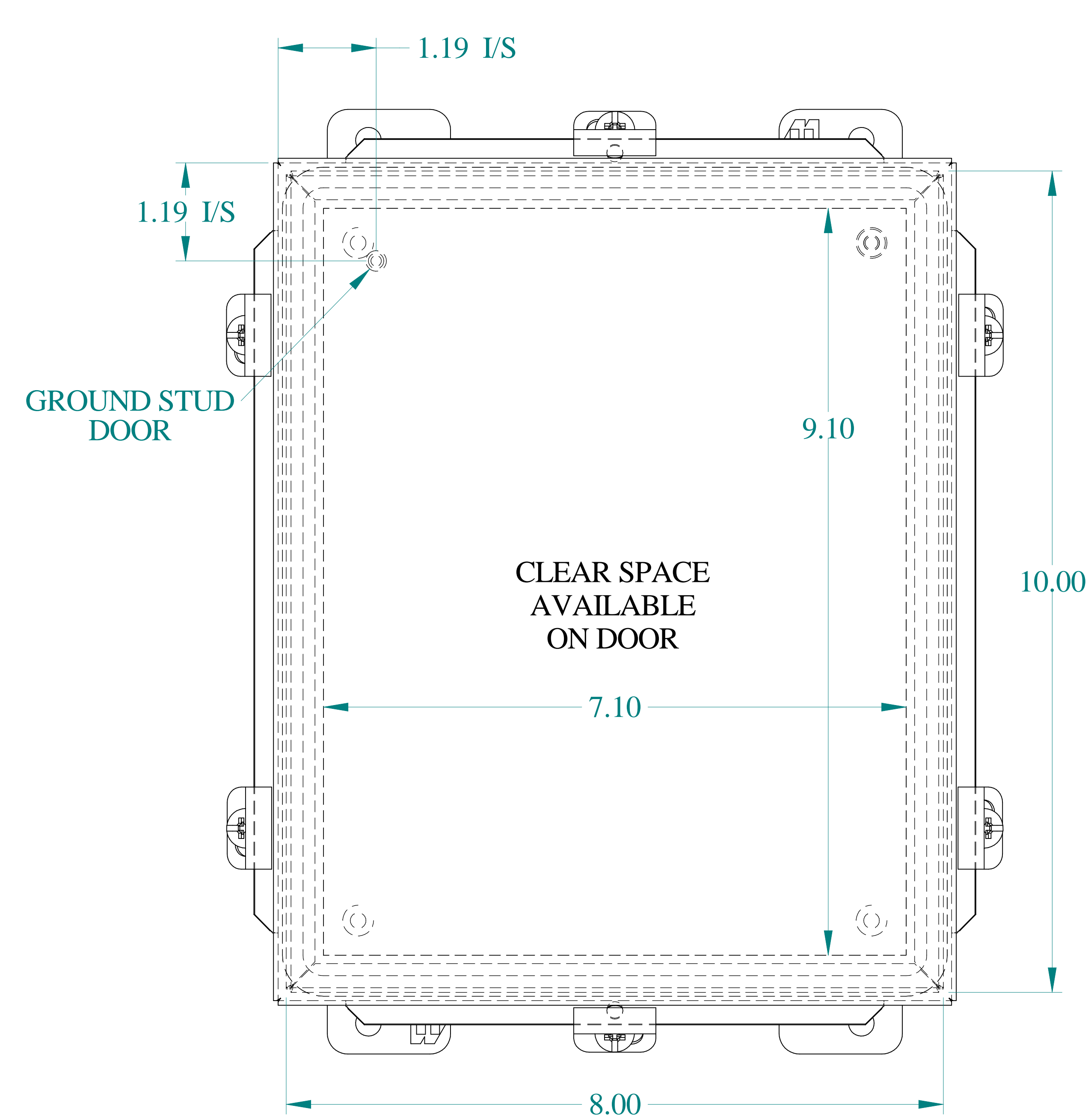
FRONT VIEW
