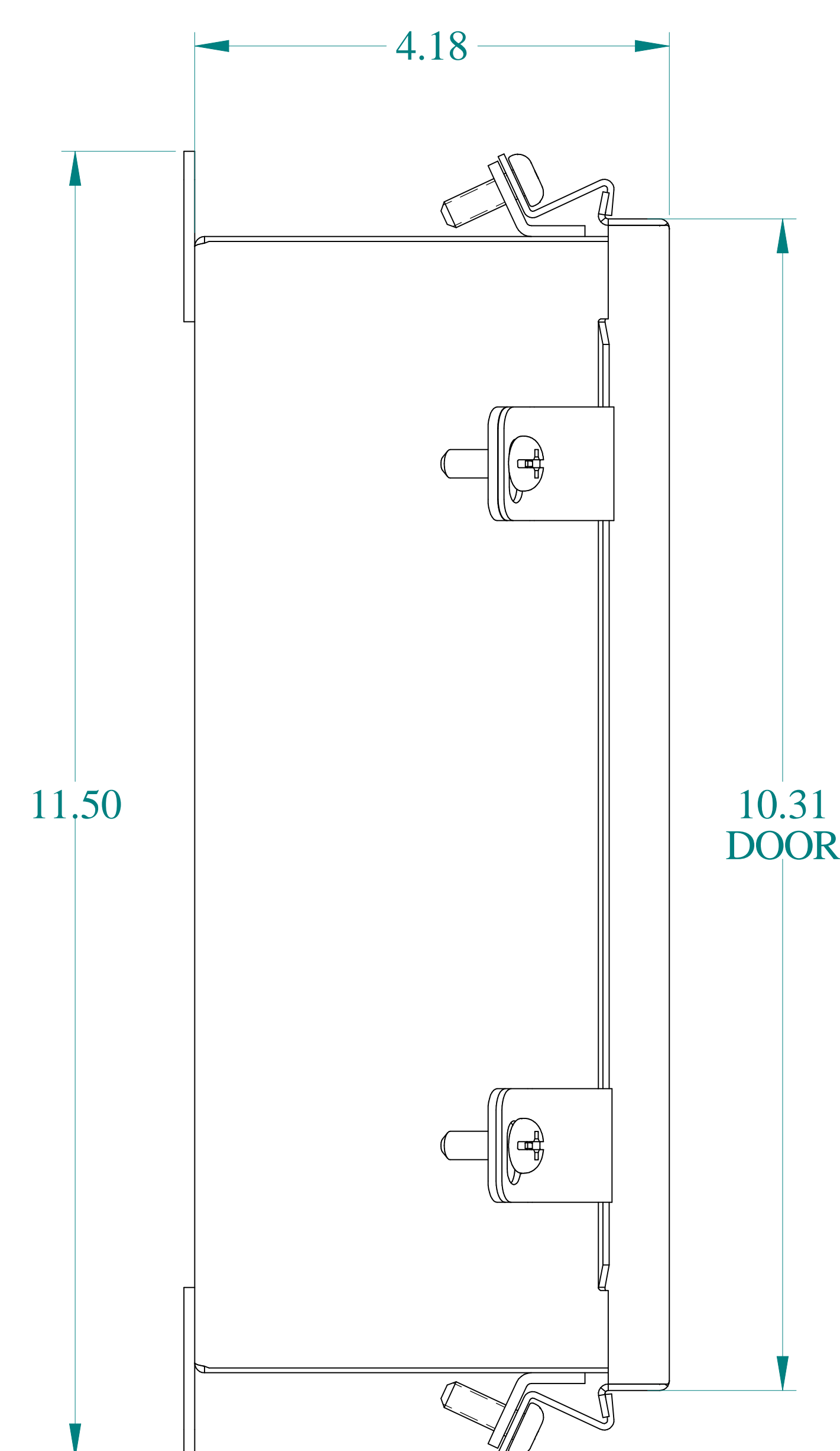
SIDE VIEW
