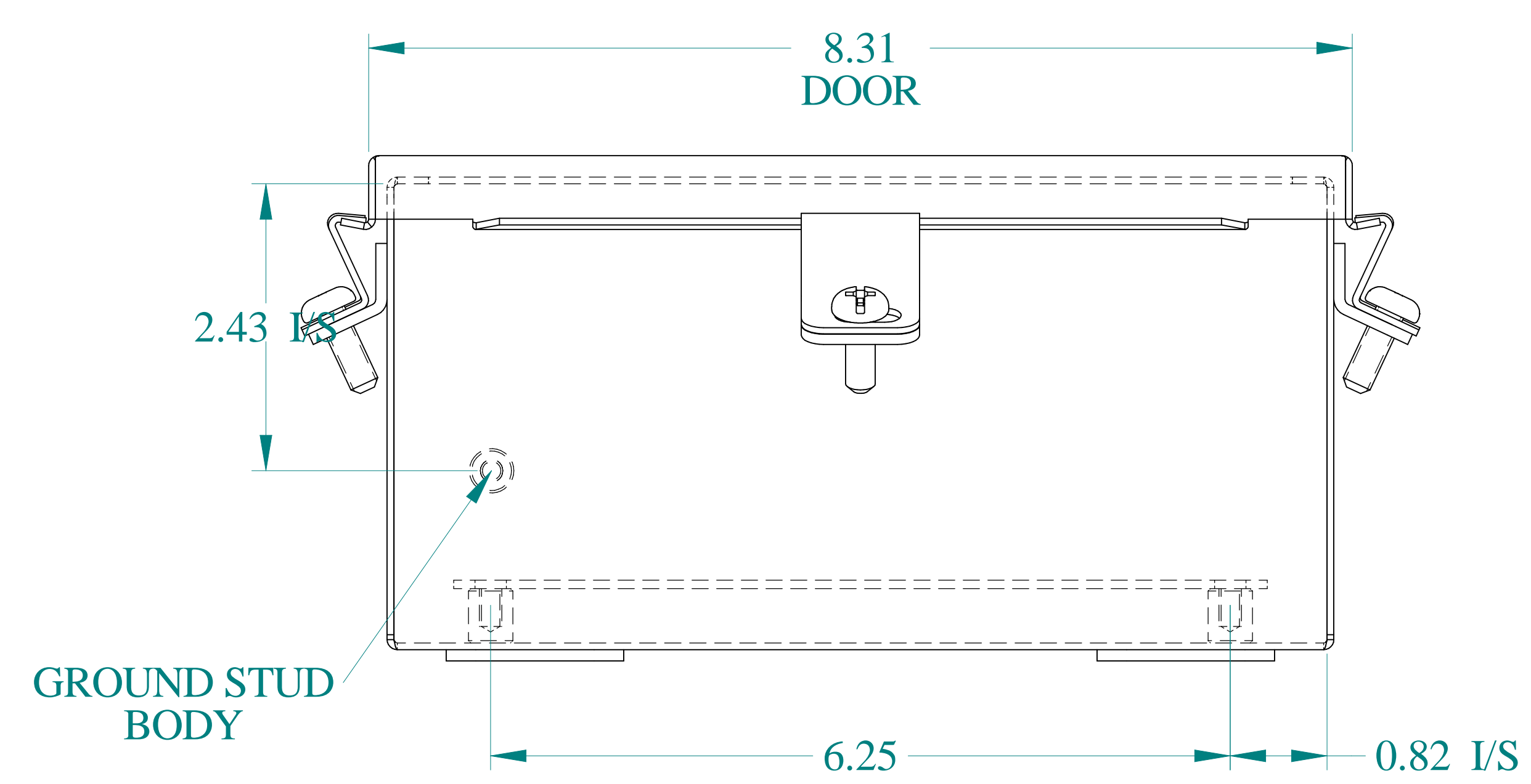
BOTTOM VIEW
