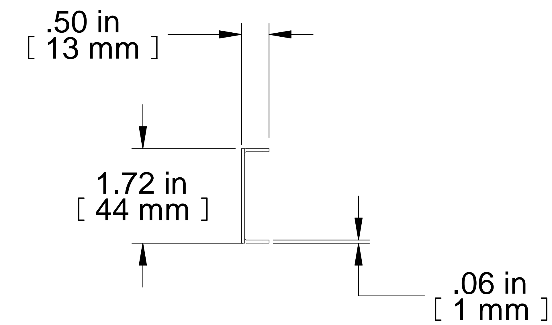
R.S. VIEW
