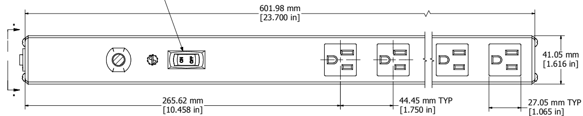
SECTION A-A (VIEW FROM FRONT)
