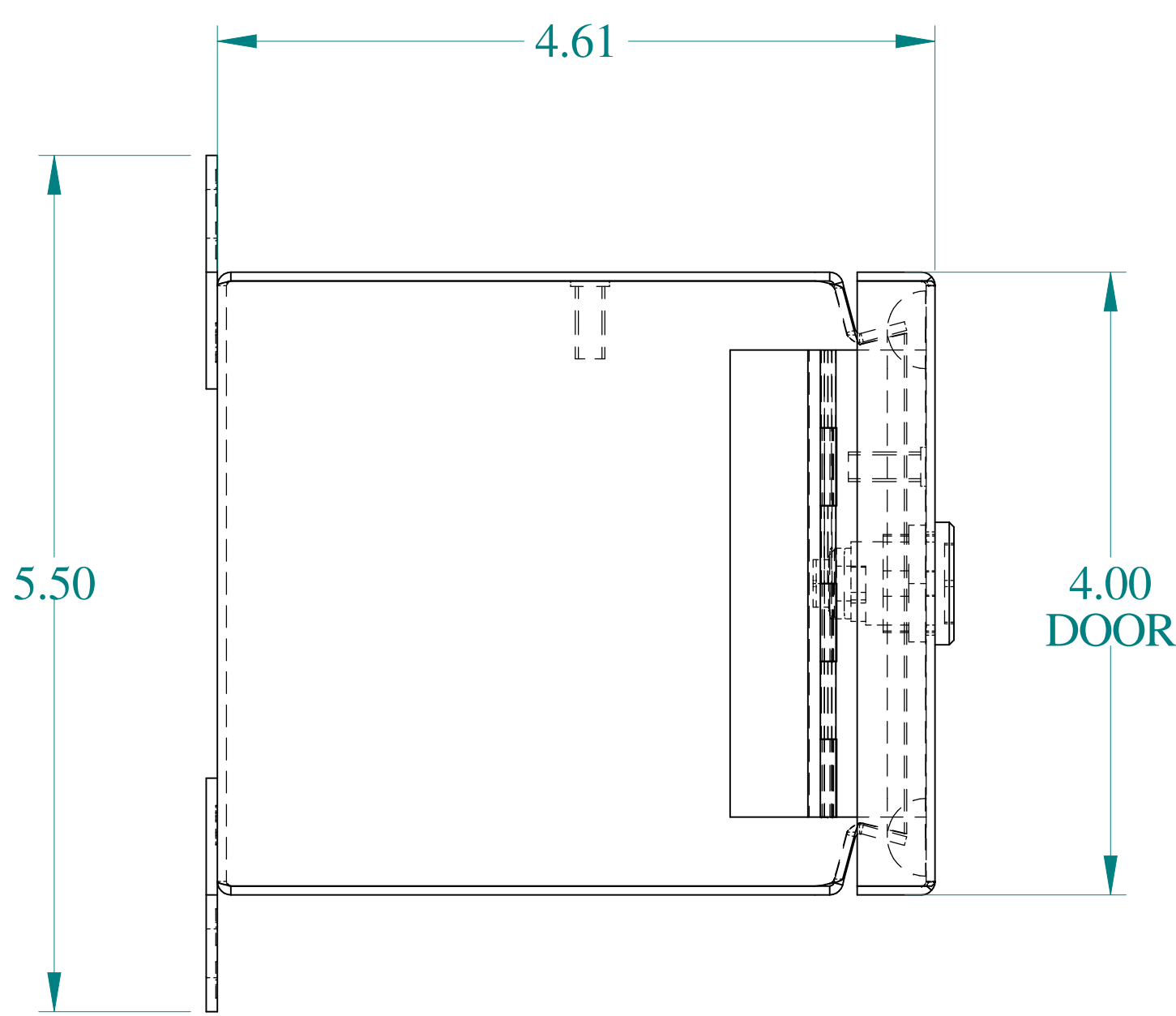
SIDE VIEW
