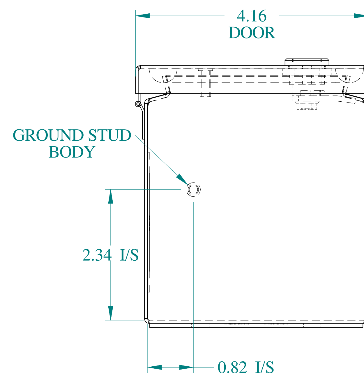
BOTTOM VIEW
