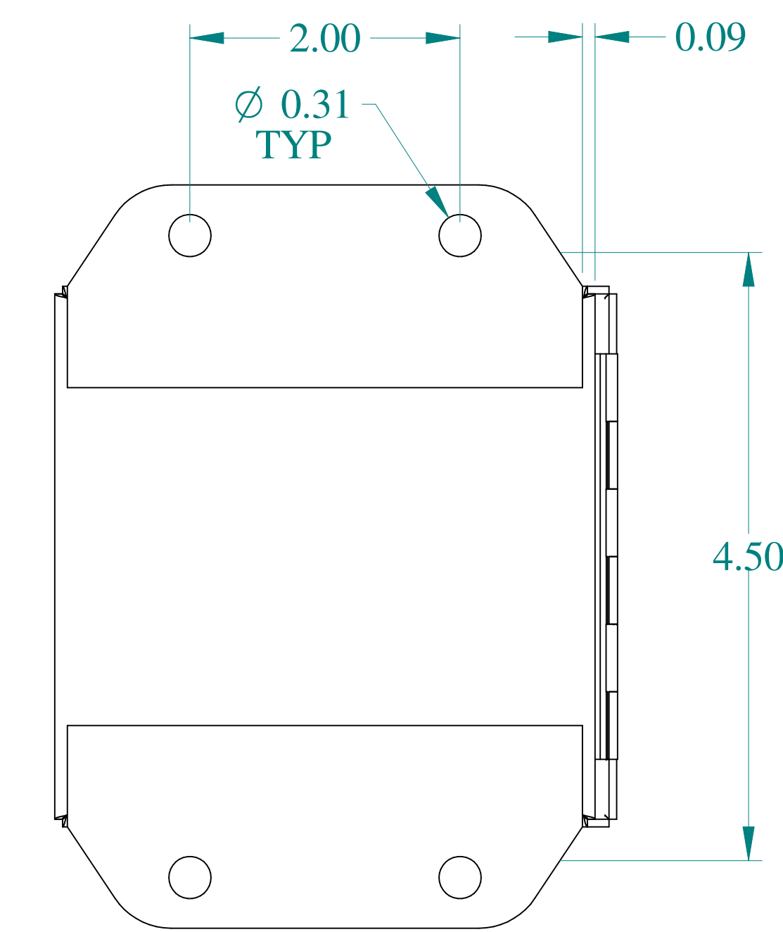
BACK VIEW
