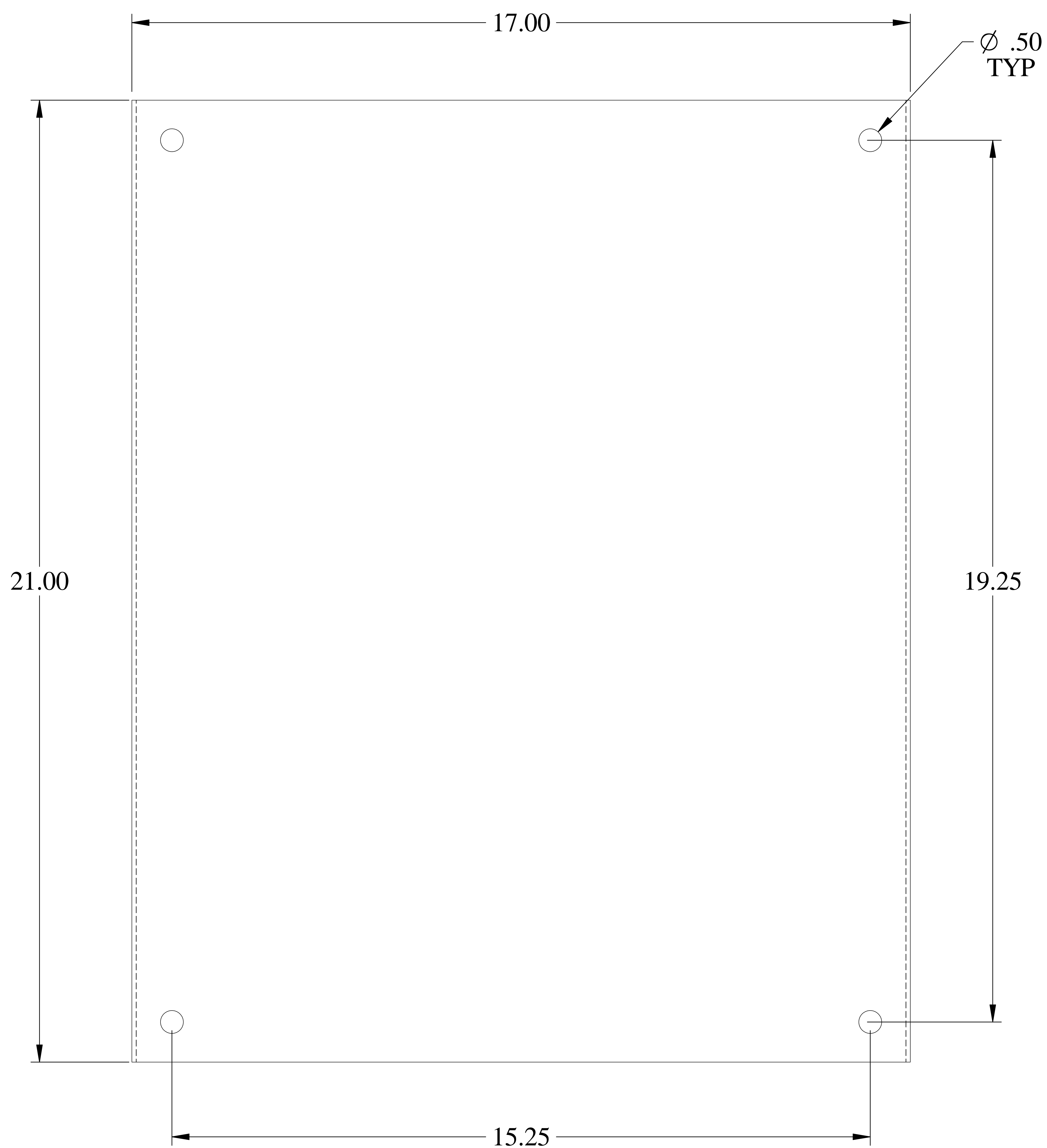
FRONT VIEW
