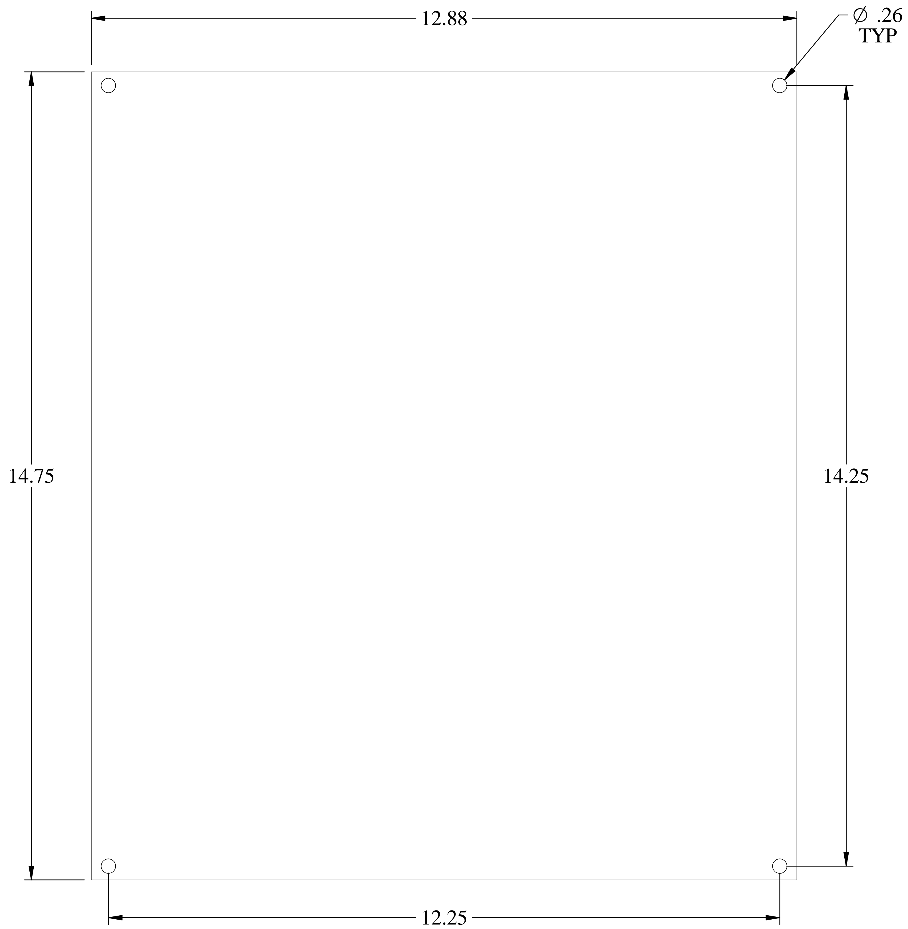
FRONT VIEW
