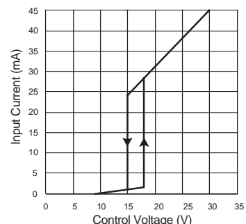
Figure 3 – XV relay
