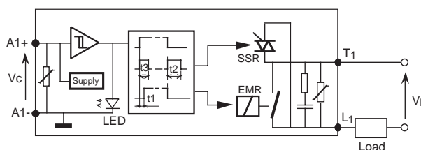
Figure 2 – XV relay
