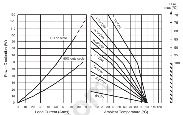
Figure 5e — 75A output current
