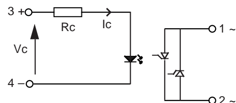
Figure 3 — LS relays
