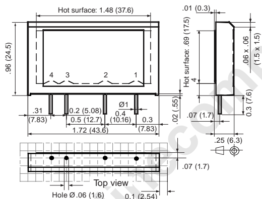
WEIGHT: 0.53 oz. (15g) TOLERANCES: ±0.01 Figure 1 — LS relays; dimensions in inches (mm) (See Figure 12 for LS with HS1)
