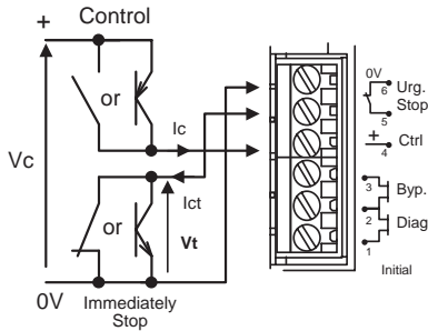
Fig. 4 HIGH SIDE CONTROL (PNP)
