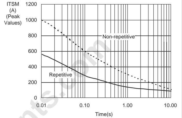
Fig. 14 OVERLOAD CURRENT CHARACTERISTIC REGARDING OVERLOAD DURATION
