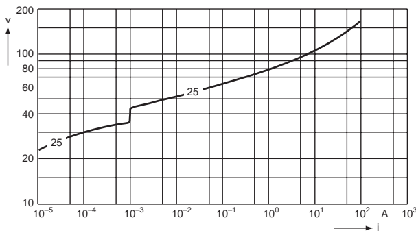
Fig. 11 STATUS OUTPUT OVERVOLTAGE PROTECTION CHARACTERISTIC
