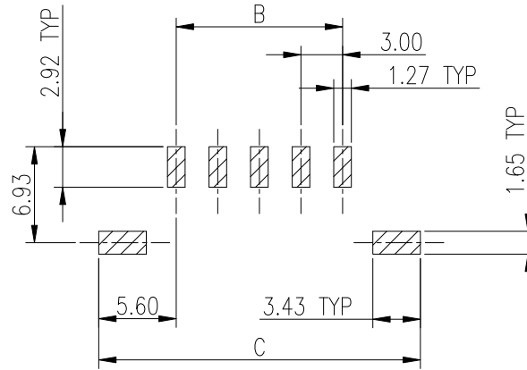
RECOMMENDED P.C.B LAYOUT (DEFAULT TOLERANCE: ±0.05)
