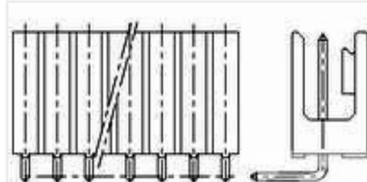
TE Part #1-969973-0 2x10P HV100 REC. CON, SMD, GOLD, BLISTER
