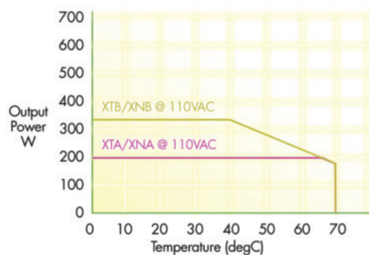
Ultra Quiet 4 slot Derating Curves
