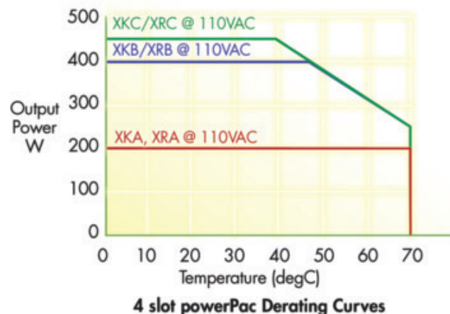
XKA/XKB/XKC and XRA/XRB/XRC @ 110VAC Derating
