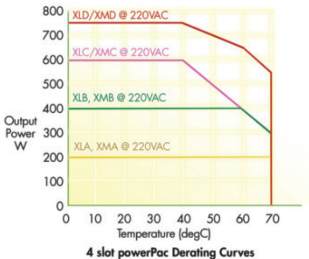
XLA/XLB/XLC/XLD and XMA/XMB/XMC/XMD @ 220VAC Derating
