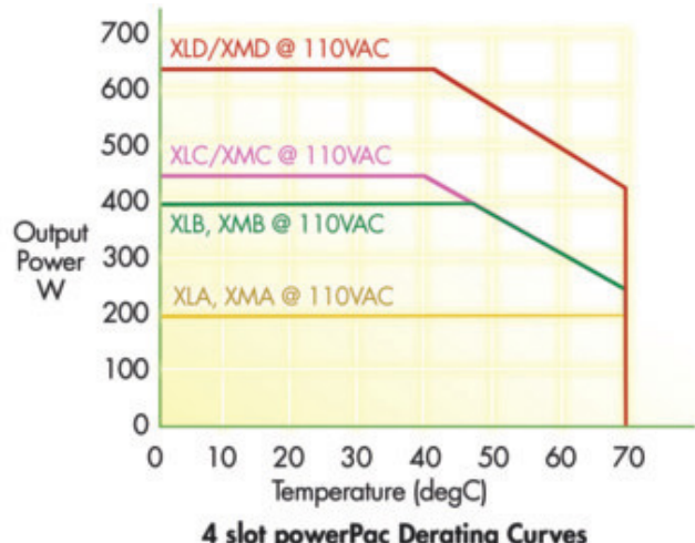
XLA/XLB/XLC/XLD and XMA/XMB/XMC/XMD @ 110VAC Derating
