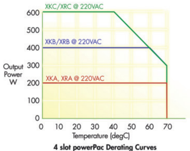
XKA/XKB/XKC and XRA/XRB/XRC @ 220VAC Derating
