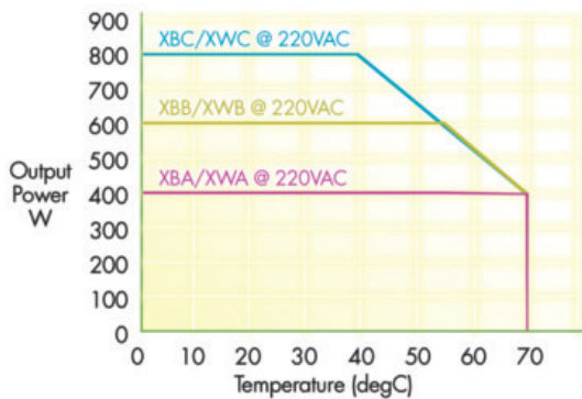
Ultra Quiet 6 slot Derating Curves
