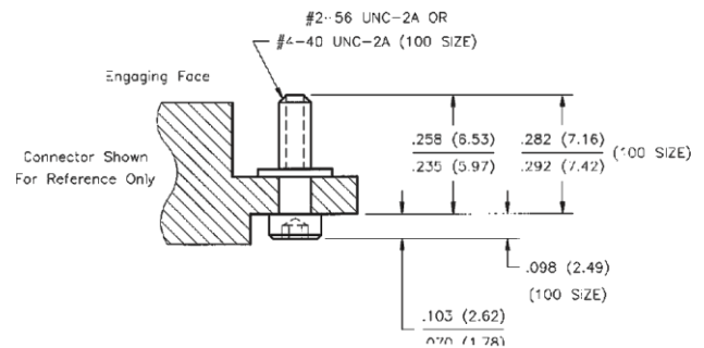
Low Profile Jackscrew
