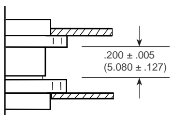
Pin and Socket Front Mounted
