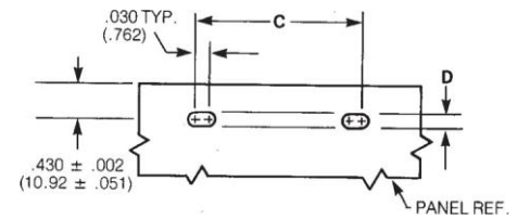
Figure 3: Edgeboard Mounting
