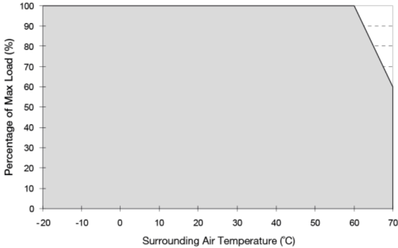
Fig. 1 De-rating for All Mounting Orientation (All Models) > 60°C de-rate power by 4% / °C
