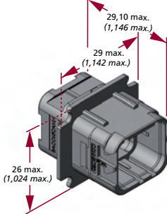
● Extender receptacle
