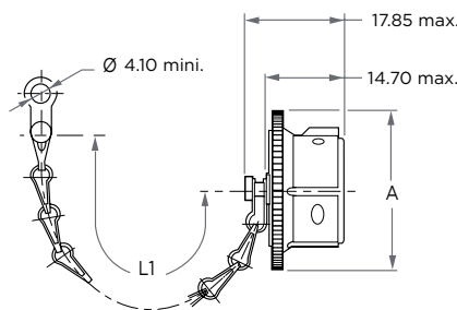
TYPE 76-70**
