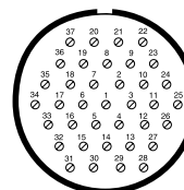
61-14 37 contacts size 16
