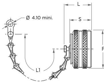
TYPE 70
