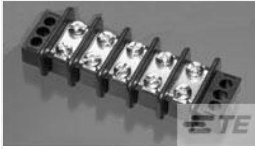
TE Part #1546307-2 2P .374" DR BARRIER, W/WASHER
