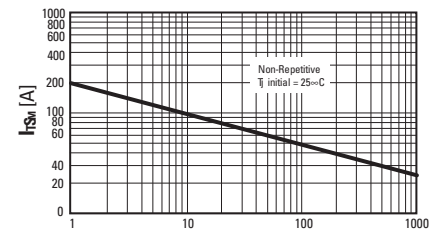
Fig. 4: Non-repetitive surge peak current versus number of cycles.
