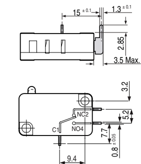
X2 for printed circuit board, rear output
