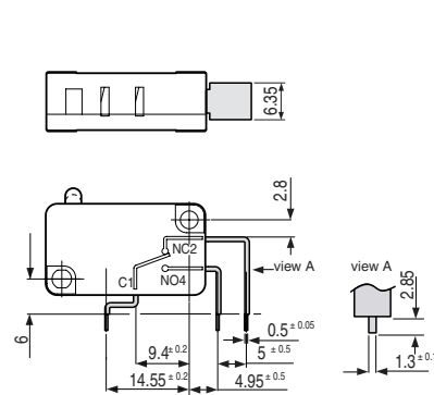
X1 for printed circuit board, straight output
