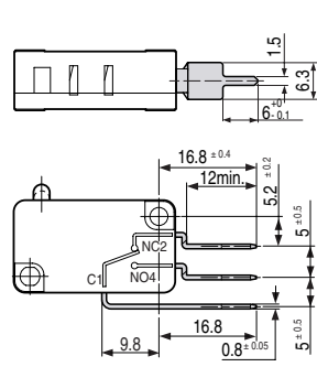
W3R2.5 for RAST 2.5 connector (SP9307)
