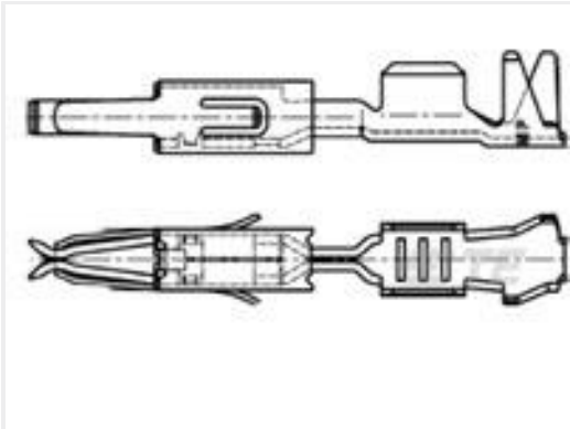
TE Part #969005-2 MT2 A REC 1.6 Contact SWS Sn
