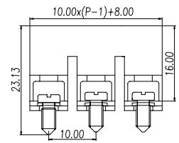
Dimensions - mm
