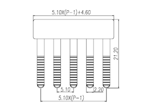
Dimensions - mm
