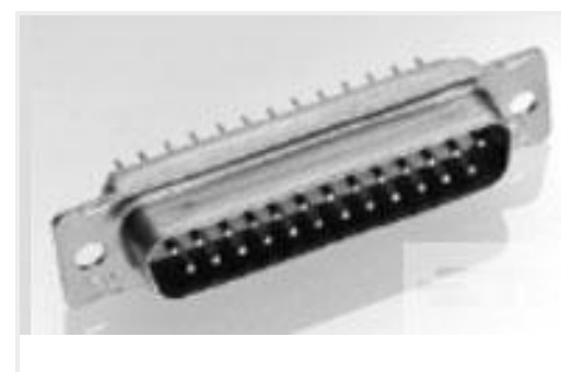
TE Part #205162-1 AMPLIMITE,ASY,PLUG,STD,109,1
