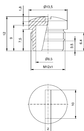
DIMENSION DRAWING
