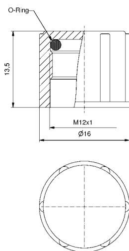
DIMENSION DRAWING
