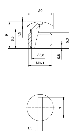
DIMENSION DRAWING
