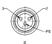
2-pos + Ground male
