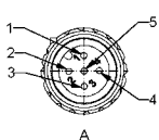
5-pos male
