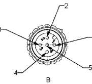
5-pos male
