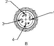
4-pos male
