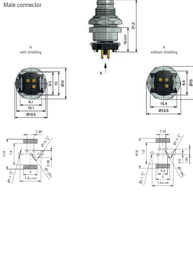
Male connector
