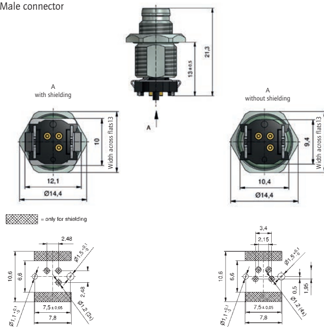
Male connector
