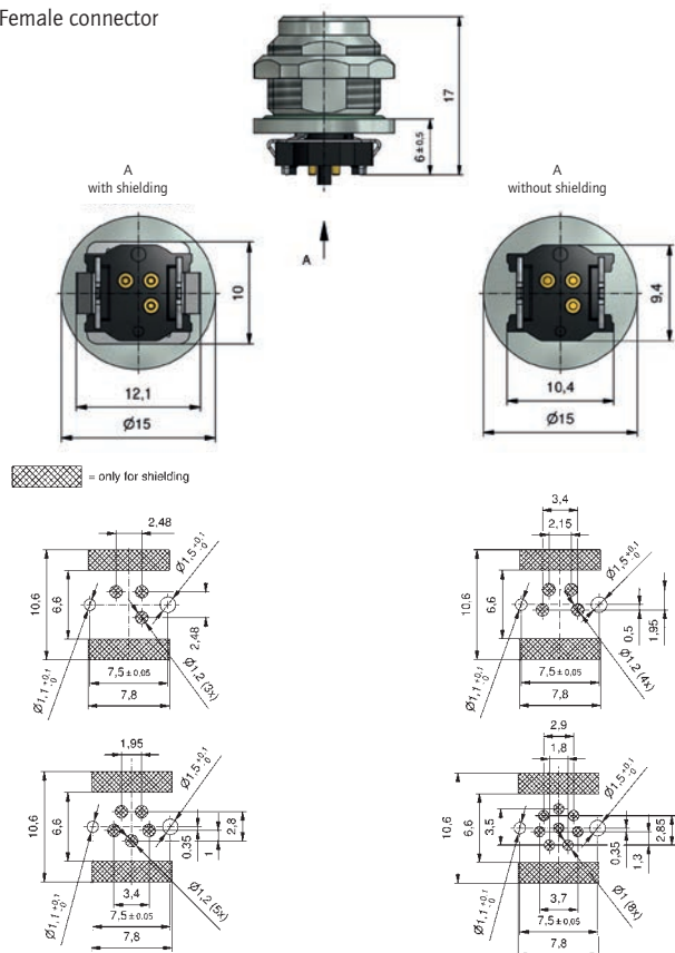
Female connector
