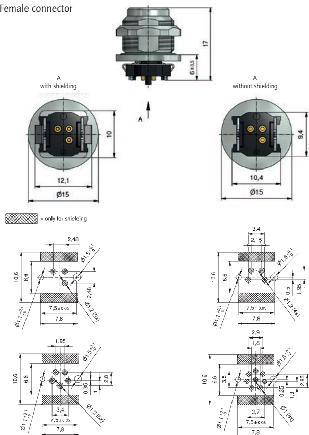
Female connector
