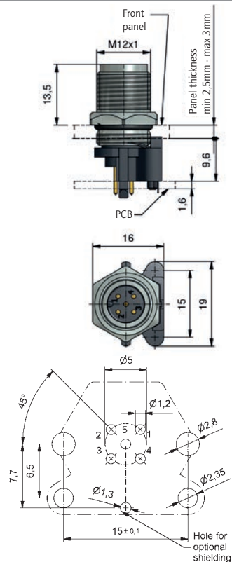
Male connector 4-5-pos. A/B/D-coded
