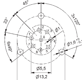
Female connector 8-pos. A-coded
