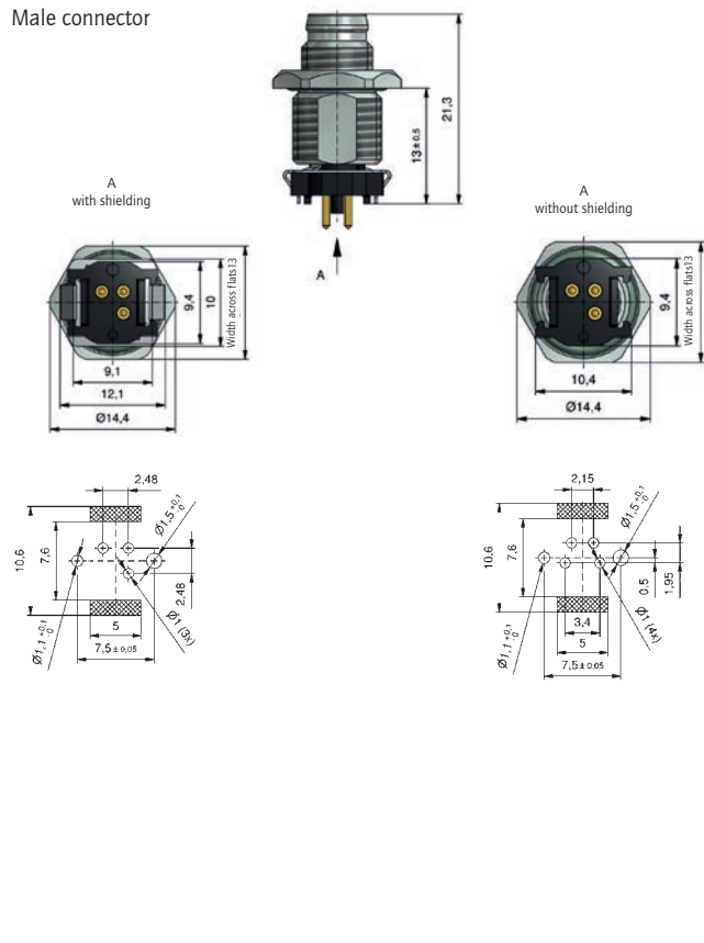
Male connector
