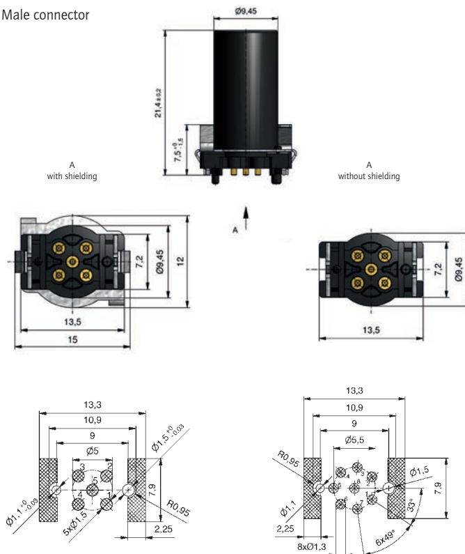
Male connector
