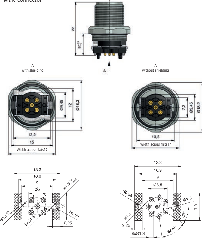
Male connector
