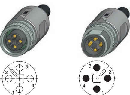
M12x1 T-coded
